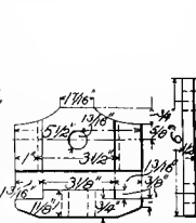
Figs. 4693-4. WASHER (2)
